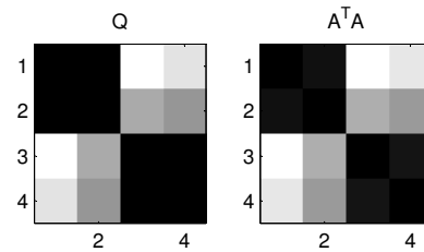
Fig. 8. \mathbf{A}^T\mathbf{A} versus \mathbf{Q} for the example in Fig. 7.
